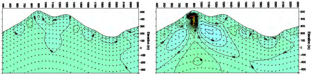
Figure 7: TE-mode SCS2D 2-D Inversion Model With Topography
