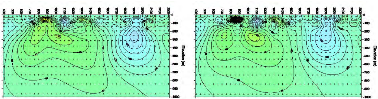
Figure 5: TM-mode SCS2D 2-D Inversion Model Without Topography
