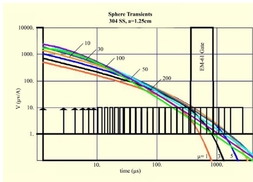
Figure 4: Receiver loop dB/dt transients versus log time. The NanoTEM system records transient values at 31 time windows spaced logarithmically between 0.1 and 2000 μsec after the transmitter current pulse. Transient shape can provide diagnostic information about UXO properties. Colored curves show the different transient responses expected from a conductive spherical object with relative permeability values ranging from 1 to 200.
