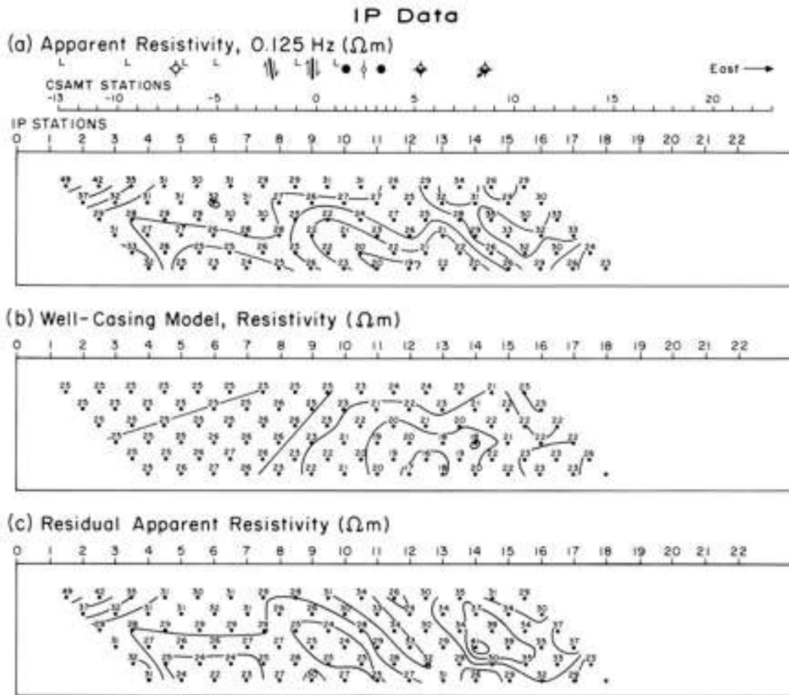
Fig. 8. Apparent-resistivity data and well-casing model results from Line 3 of the IP survey at Trap Spring. See text for details on the well-casing model. The top shows CSAMT and IP station numbers, faults, wells, a surface pipeline (small circle with a vertical bar), and surface lineaments from air photos ('L').
