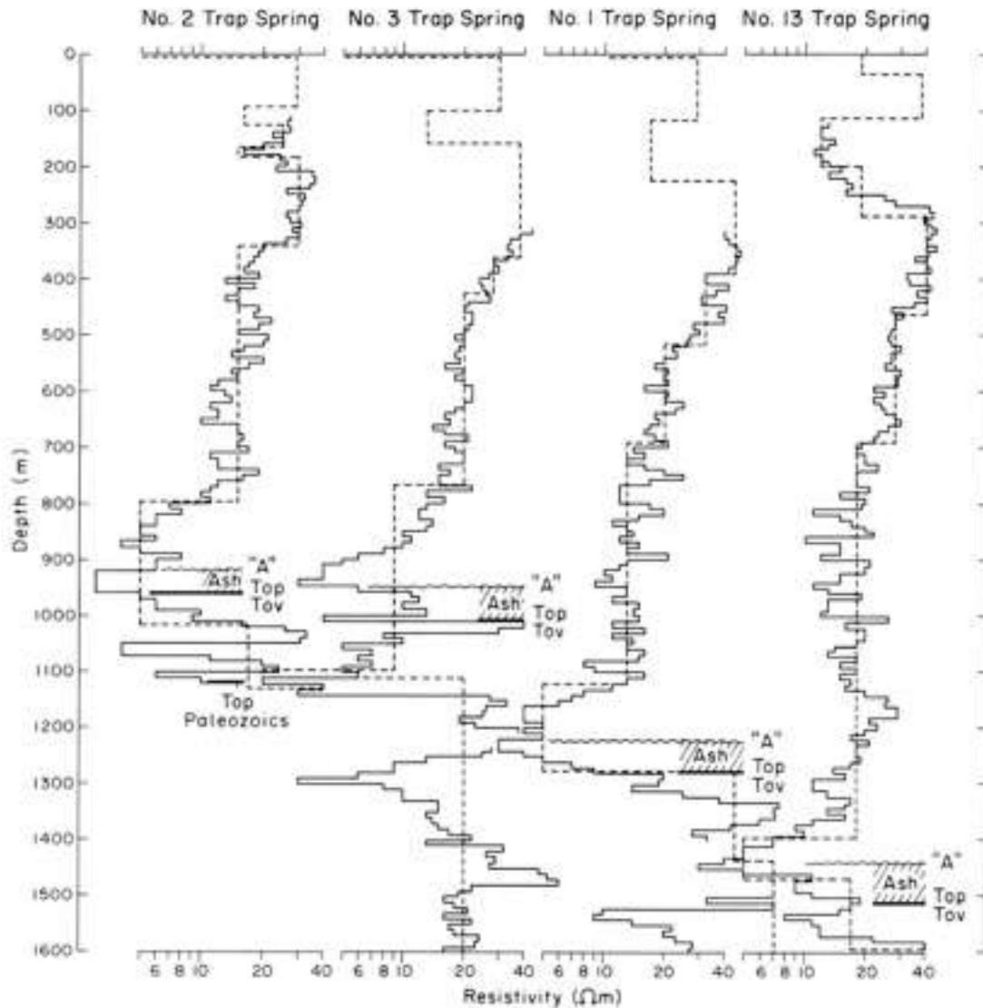
Fig. 11. Digitized deep-induction logs for Trap Spring Field. Dotted lines indicate the simplified layered models used to forward-model the CSAMT data, as described in the text. Note that the logs do not start from the surface, necessitating the insertion of surficial layers required for the modelling.
