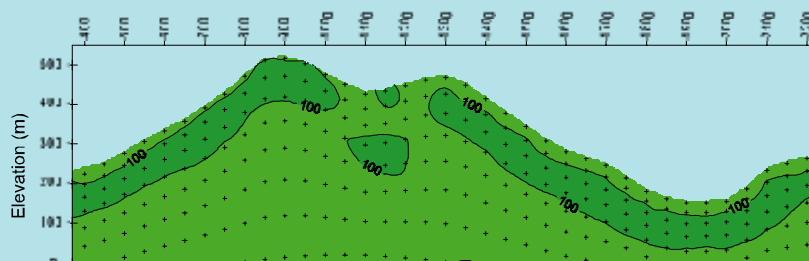
Figure 4: Inversion of data from the pseudosection in Figure 2, with topography.
